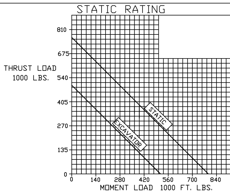
CHART BASED ON STATIC RADIAL (RAKING) LOAD OF 181800 LBS.
